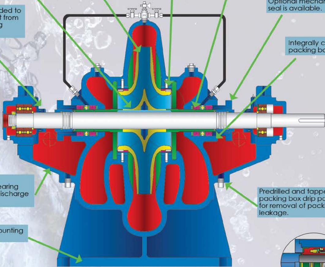
Patterson PRG Mechanical Seal
