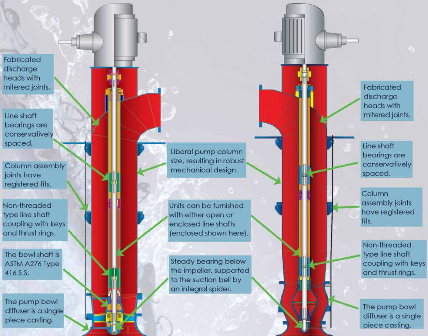
Available in open or enclosed line shaft configurations. Enclosing tubes, when used, are schedule 80 and are supported by spiders when required by the pump length.
